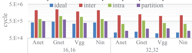
Figure 7. Comparison of execution time of layer Conv-1
