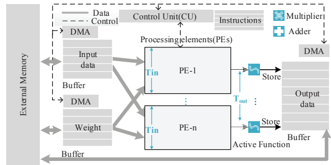
Figure 2. Architecture of a typical deep learning accelerator
