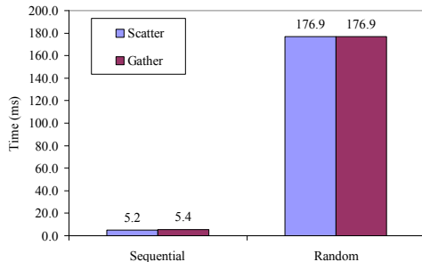
Figure 1. The elapsed time of the scatter and the gather on a GPU. Both operations underutilize the bandwidth for random locations.
