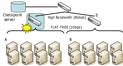
図 5 Frequent physical fault model
