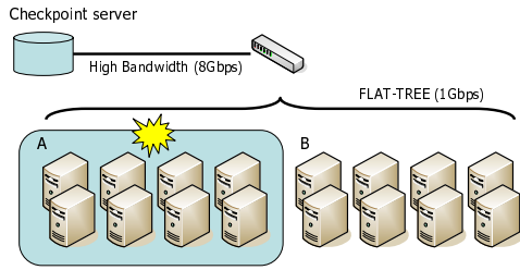
図 3 Frequent process fault model
